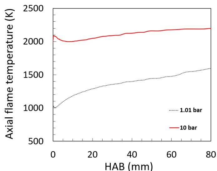
Figure 4. Centerline flame temperature (K) in function of HAB (mm) of premixed flame \text{C}_2\text{H}_4/\text{air} \phi = 1.77 at atmospheric pressure (dotted line) and 10 bar (solid line).
