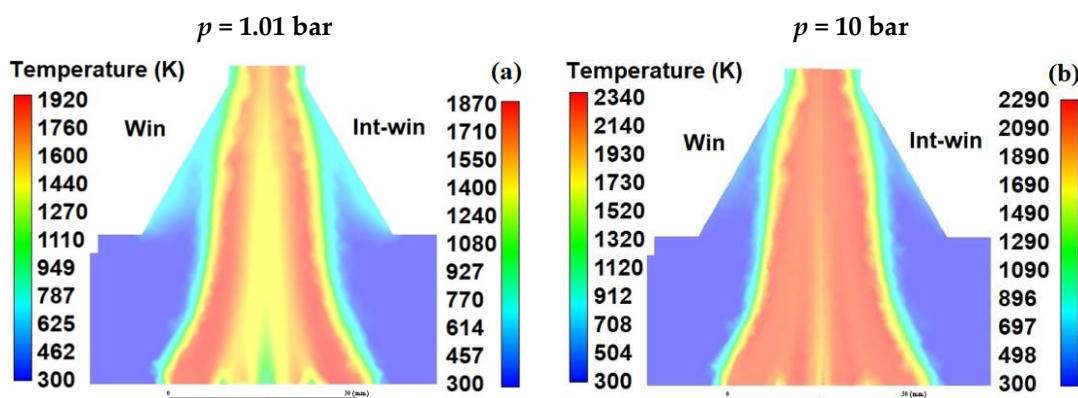
Figure 3. Temperature cross-sectional distributions (K) along window (Win) and inter-window (Int-win) axes of burner of premixed flame \text{C}_2\text{H}_4/\text{air} \phi = 1.77 at atmospheric pressure (a) and 10 bar (b).
